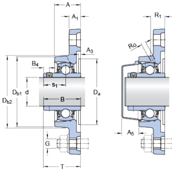
skf fytb 25 tf bearing
